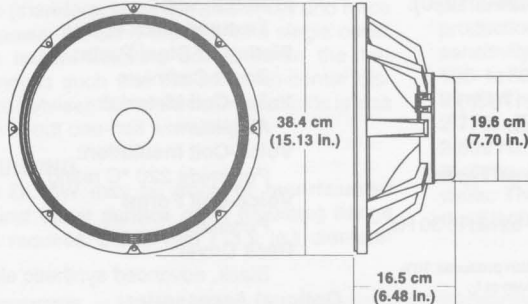
FIGURE 5 — Dimensions
